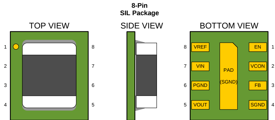
Pin Functions
