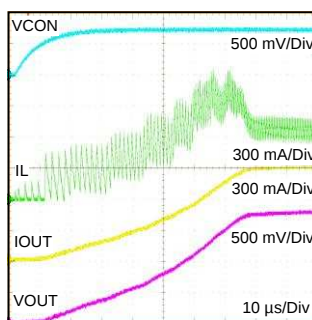
Figure 9. Startup Behavior of Current Limit Based Softstart.
