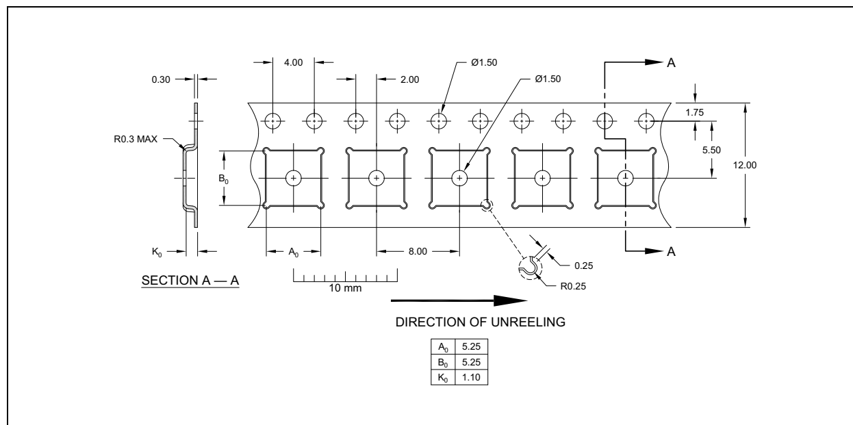
FIGURE 9-2: QFN, 5X5 TAPING DIMENSIONS AND PART ORIENTATION
