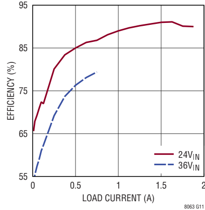
Efficiency, V_{OUT} = 15\text{V}
