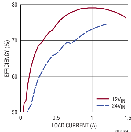
Efficiency, V_{OUT} = -8\text{V}
