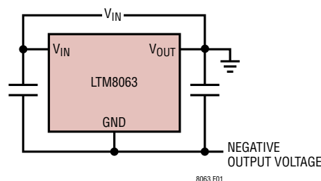
Figure 1. The LTM8063 Can Be Used to Generate a Negative Voltage
