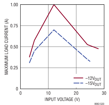
Maximum Load Current vs V_{IN}
