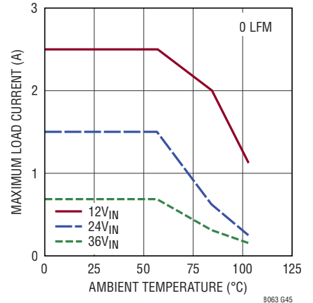
Derating, V_{OUT} = 8\text{V} , DC2494A Demo Board
