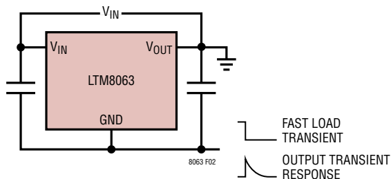
Figure 2. Any Output Voltage Transient Appears on LTM8063 GND
