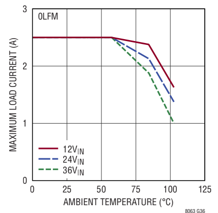
Derating, V_{OUT} = 1.2V , DC2494A Demo Board
