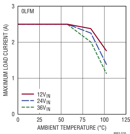
Derating, V_{OUT} = 1V , DC2494A Demo Board
