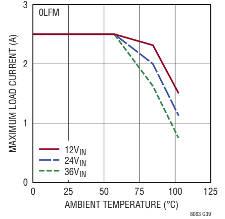
Derating, V_{OUT} = 2\text{V} , DC2494A Demo Board
