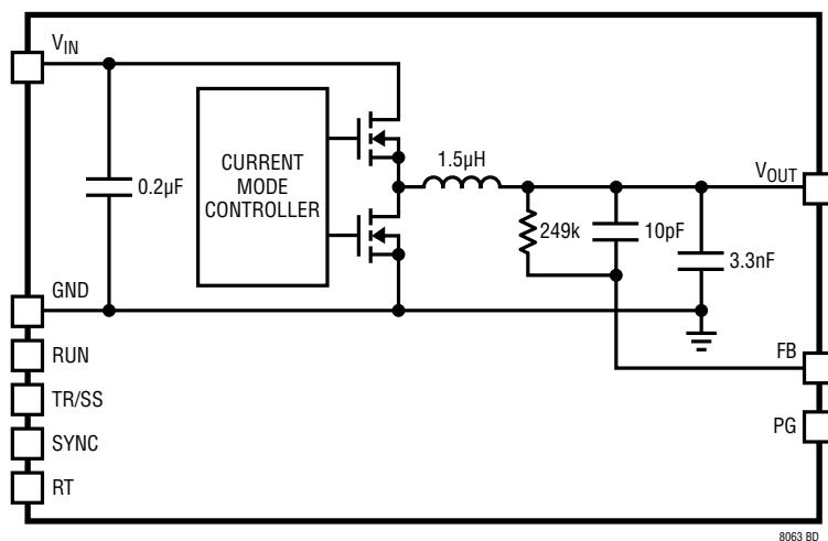
LTM8063 Block Diagram
