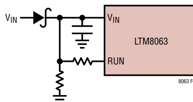
Figure 4. The Input Diode Prevents a Shorted Input from Discharging a Backup Battery Tied to the Output. It Also Protects the Circuit from a Reversed Input. The LTM8063 Runs Only When the Input Is Present
