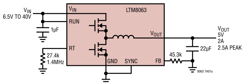
5V OUT from 6.5V IN to 40V IN Step-Down Converter
