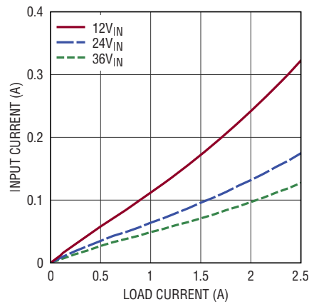
Input vs Load Current, V_{OUT} = 1\text{V}
