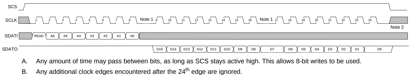
Figure 24. SDF Timing Diagram 2
