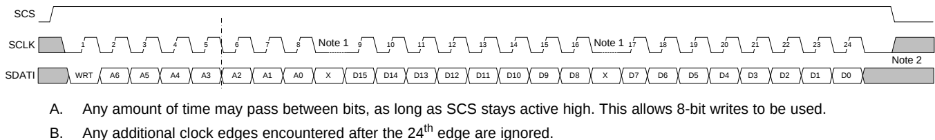
Figure 23. SDF Timing Diagram 1
