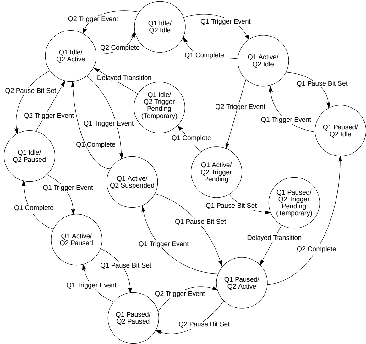
Figure 28-12. Queue Status Transition
