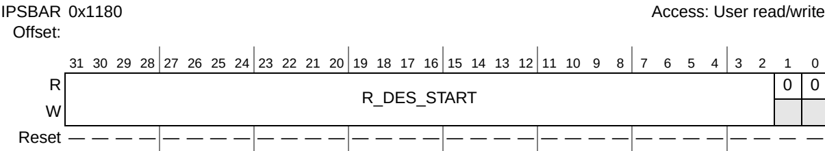
Figure 17-22. Ethernet Receive Descriptor Ring Start Register (ERDSR)
