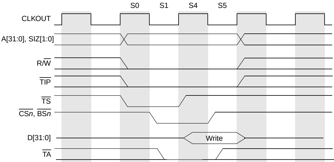
Figure 13-10. Write Cycle with Fast Termination
