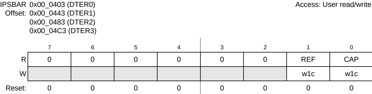
Figure 21-4. DTERn Registers
