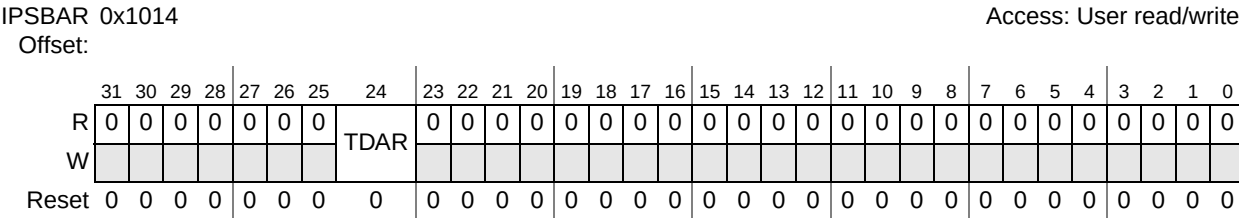
Figure 17-5. Transmit Descriptor Active Register (TDAR)
