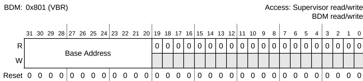
Figure 2-7. Vector Base Register (VBR)
