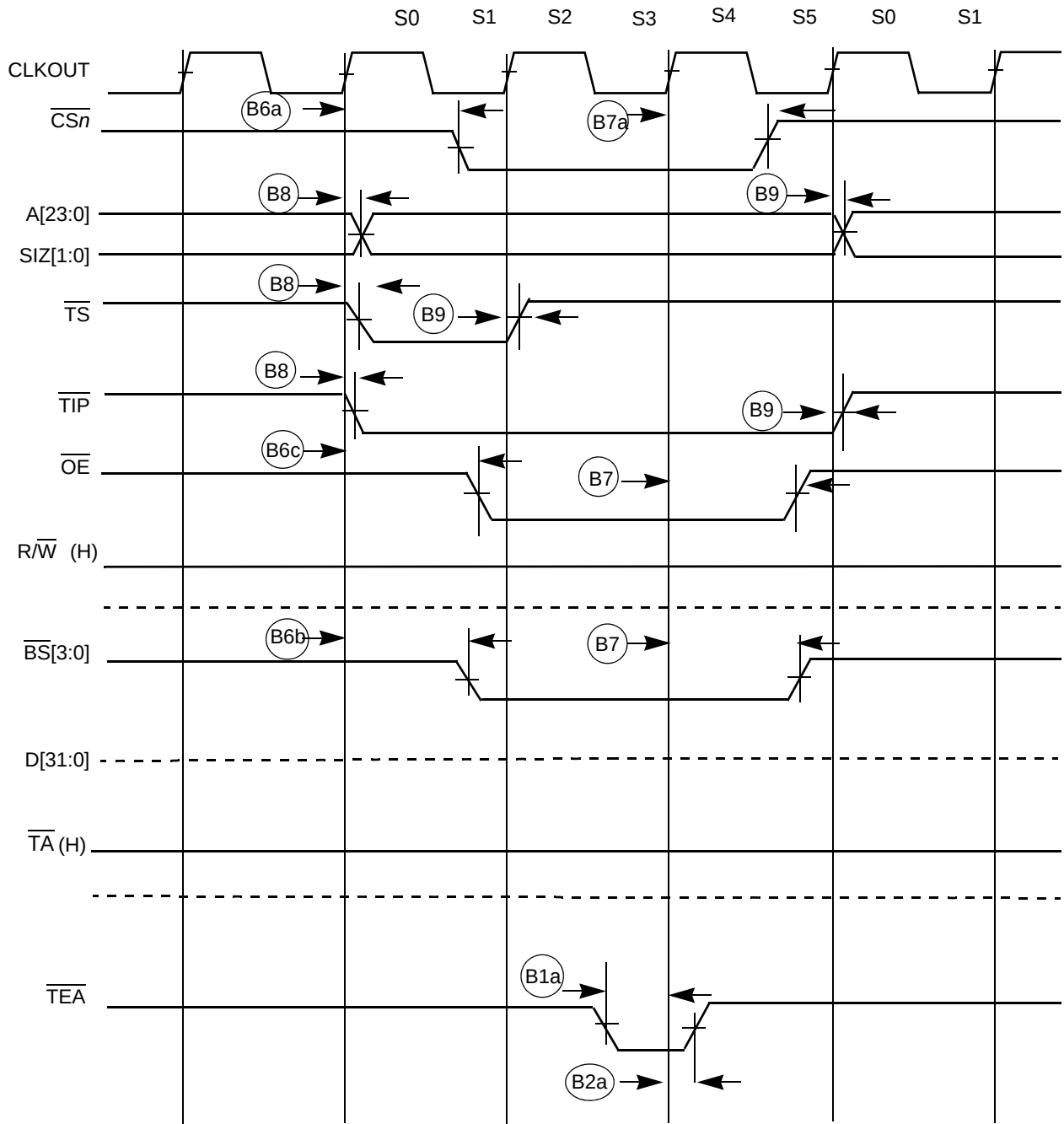
Figure 33-5. Read Bus Cycle Terminated by \overline{\text{TEA}}
