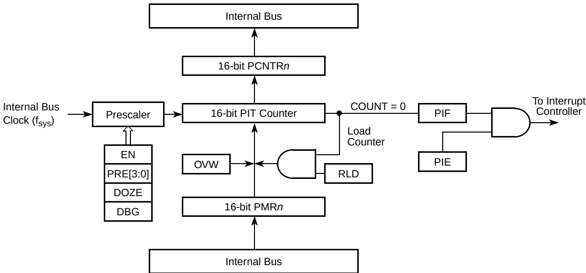
Figure 19-1. PIT Block Diagram
