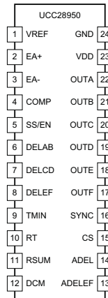
PW Package 24-Pin TSSOP Top View
