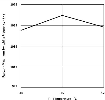
Figure 12. Maximum Switching Frequency vs Temperature
