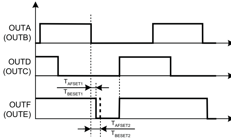
Figure 31. Delay Definitions Between OUTA and OUTF, OUTB and OUE
